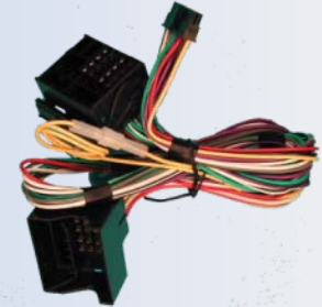
Vehicle Specific Harness (EVH-xxx)
