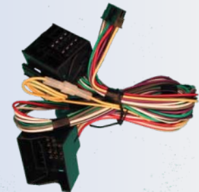
Elan Vehicle Specific Harness (EVH-xxx)
